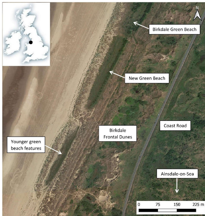
Fig. 5. Aerial photo of southern Green Beaches in 2020. “Younger Green Beach features” includes ‘Newest’ and ‘Even Newer Green Beaches’
