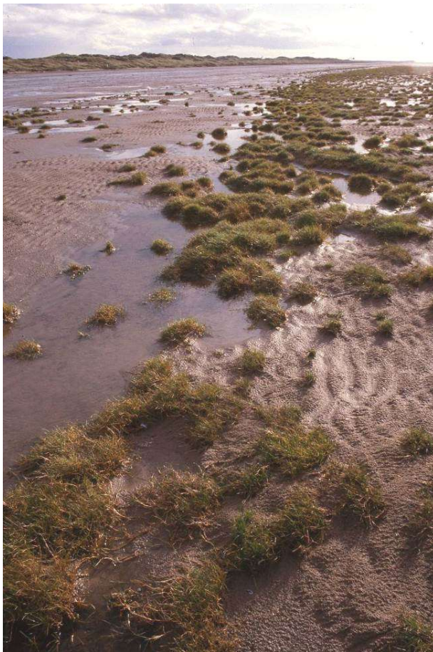
Fig. 1. Early stage in Green Beach formation, Birkdale 1987
